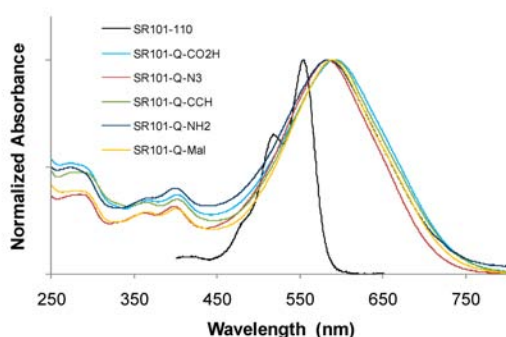
Figure 2. Absorption data of SR101-Q-X in PBS at 25 °C. a Isolated yields after purification by semipreparative RP-HPLC. Each quencher compound was recovered with a purity up to 99%.
