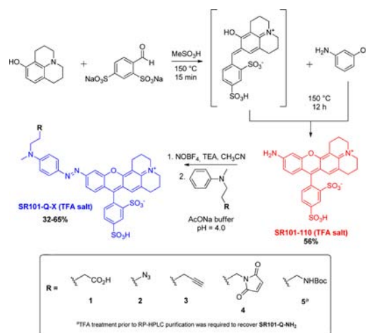
Scheme 1. Synthesis of Azo-sulforhodamine Hybrids SR101-Q-X
