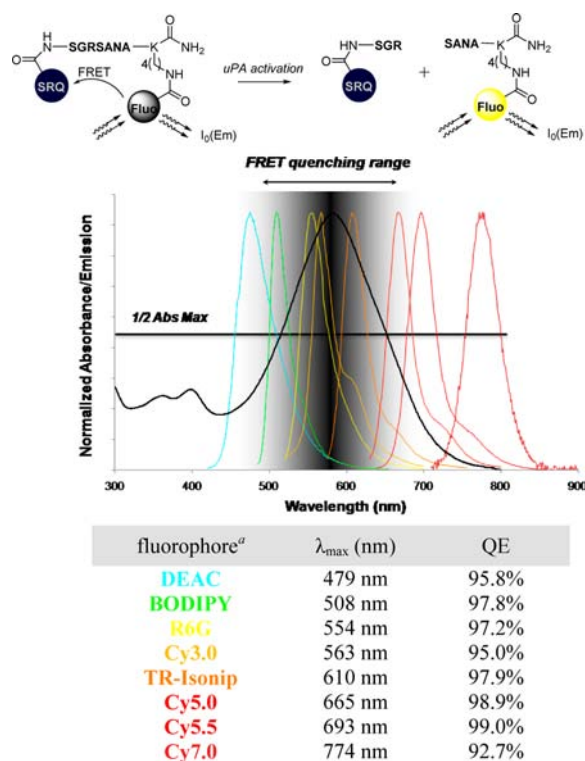
Figure 3. Fluorescence quenching range of SR101-Q. a DEAC = 7- N,N -diethylaminocoumarin, R6G = rhodamine 6G, and TR-Isonip = Texas Red-isonipetric acid; see SI for the chemical structures of fluorophores. b Fluorescence emission measurements were performed in PBS at 25 °C before and after enzymatic digestion with uPA.
