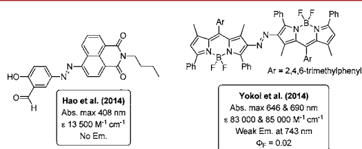
Figure 1. Nonfluorescent azo dyes derived from fluorescent anilines and recently reported in the literature.
